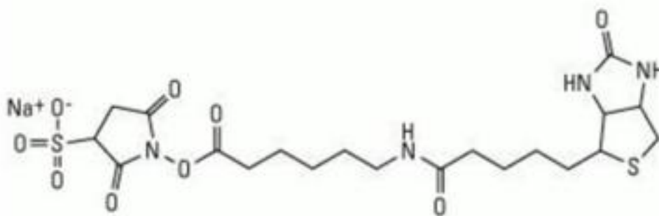
Sulfo-NHS-LC-Biotin
