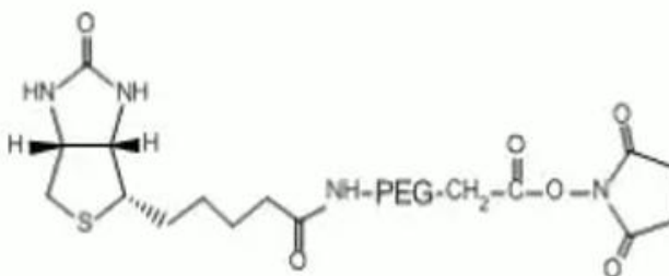
Biotin-PEG-NHS
